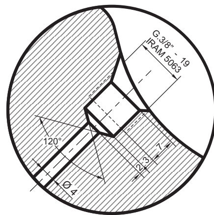
DETALLE "1"
