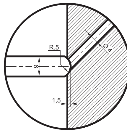
DETALLE "2"
