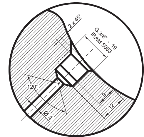
DETALLE "1"
