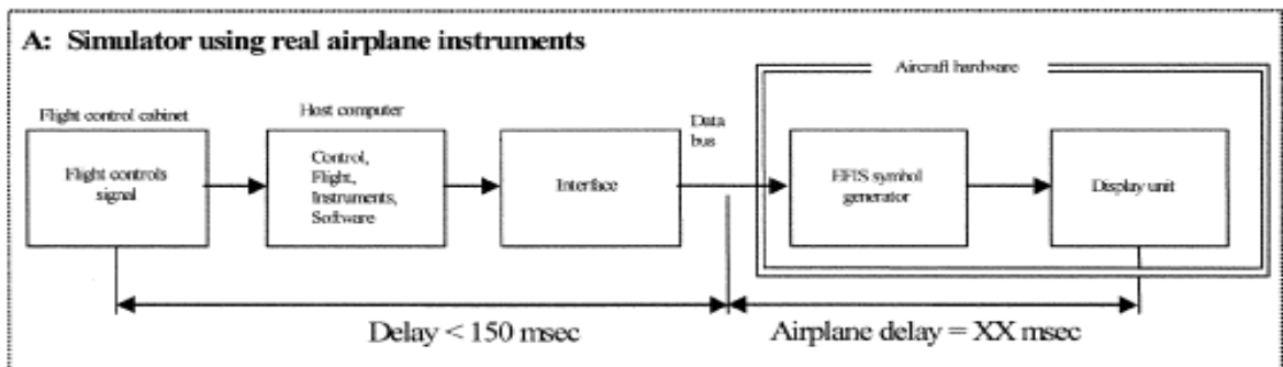
Figuras 1-IIF(A) y 1-IIF(B) – Transport delay for simulation of airplane using real or re-hosted instrument drivers
