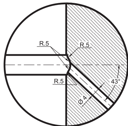
DETALLE "2"
